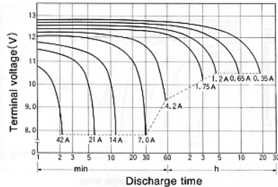
Discharge characteristics(0°C(32°F))
