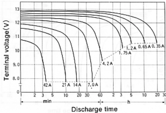
Discharge characteristics(25°C(77°F))
